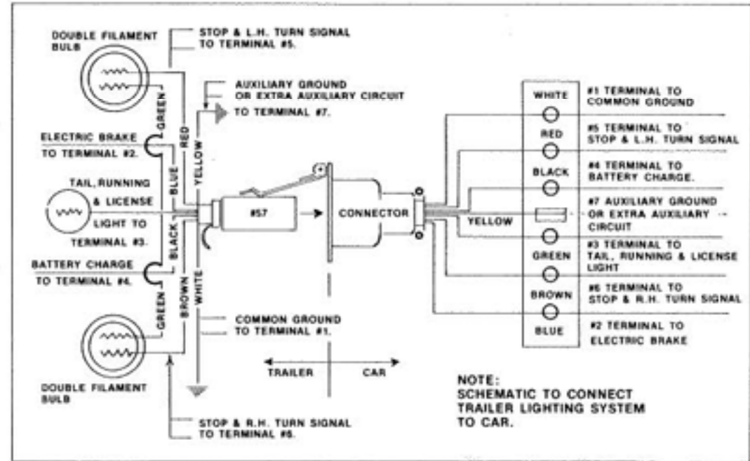
#57 7-CIRCUIT DIAGRAM
